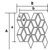
Diamond Mosaic A 14 5 / 9 " B 12 6 / 7 " a 11 2 / 3 " b 11 2 / 3 " c 2.9" x 1.6" d 5.7" x 2.3"
