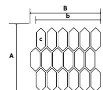
Picket Mosaic A 12 2 / 7 " B 11 5 / 7 " b 11 5 / 7 " c 4.7" x 1.9"
