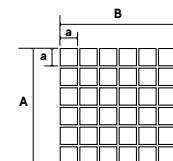
Mosaic A 11 3 / 4 " B 11 3 / 4 " a 2"
